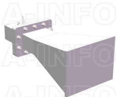
LB-340-10-C-SFSPO Standard Gain Horn Antenna 2.2-3.3GHz 10dB Gain SMA Female
